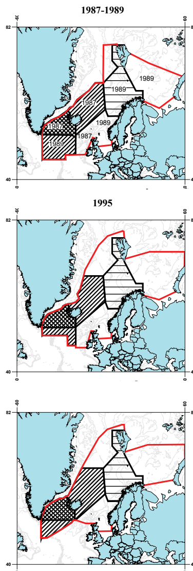
Fig. 3. Regions used in examining trends in fin whale abundance. Survey year is indicated for the 1987-1989 compilation. The Norwegian sector of the 2001 survey was surveyed in the period 1996-2001. Cross hatched – WEST; Diagonally hatched – EGI; Horizontally hatched – NORWAY; TOTAL outlined in red.
