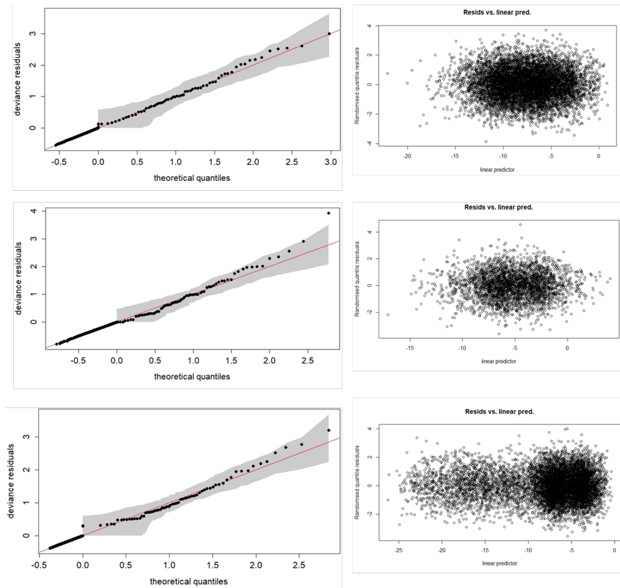
Figure S1. QQ and residual plots for the three best fitting models. Top row – full model, middle row – early simple model and bottom row – late simple model.
