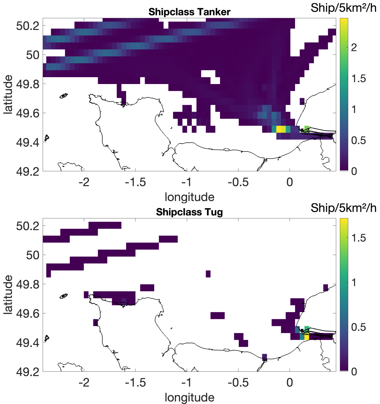
Supplementary file 4: Density map of ships with AIS transmitters recorded during 2020-2021 and 2023-2024 periods. The map represents the mean hourly count of AIS ships per 5km 2 cell. Each map represents a ship class.
